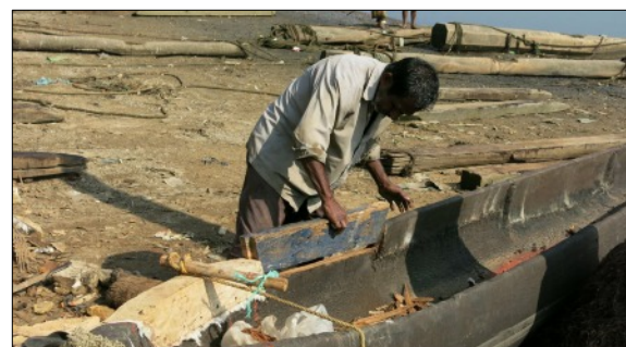
Figure 2. Monoxyllous craft used on Goa's rivers. They are so heavily coated in dikh that sewn portions are difficult to detect: a) upturned with booms still attached. Assolna; b) under repair on the slip at Cavelossim. Author.
